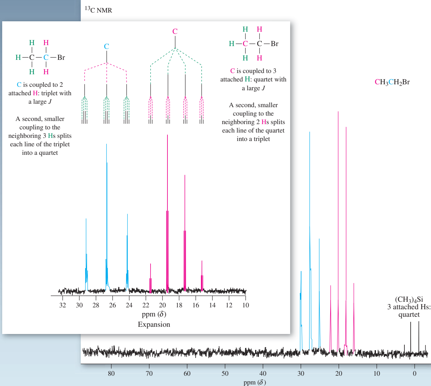
Figure 10-30 13 C NMR spectrum of bromoethane, showing the complexity of 13 C–H coupling. There is an upfield quartet ( \delta = 18.3 ppm, J = 126 Hz) and a downfield triplet ( \delta = 26.6 ppm, J = 151 Hz) resonance for the two carbon atoms. Note the large chemical-shift range. Tetramethylsilane, defined to be located at \delta = 0 ppm as in 1 H NMR, absorbs as a quartet ( J = 118 Hz) because of coupling of each carbon to three equivalent hydrogens. The inset shows a part of the spectrum expanded horizontally to reveal the fine splitting of each of the main peaks that is due to coupling of each 13 C to protons on the neighboring carbon. Thus, each line of the upfield quartet (red) is split again into a triplet with J = 3 Hz, and each line of the downfield triplet (blue) is split again into a quartet with J = 5 Hz.
