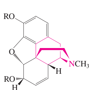
Morphine (R = H)
