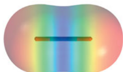
Carbon dioxide
