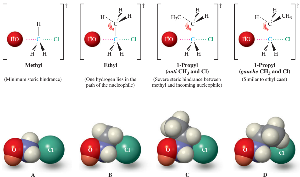
Figure 6-9 Hashed-wedged line and space-filling drawings of the transition states for S_N2 reactions of hydroxide ion with (A) chloromethane; (B) chloroethane; and (C and D) two conformers of 1-chloropropane: (C) anti and (D) gauche . Steric interference is illustrated strikingly in the space-filling drawings. Partial charges have been omitted for clarity. (See Figure 6-3.)
