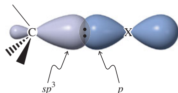
Figure 6-1 Bond between an alkyl carbon and a halogen. The size of the p orbital is substantially larger than that shown for X = \text{Cl, Br, or I} .
