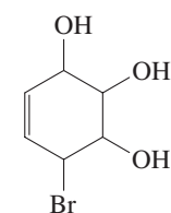
Bromoconduritol
