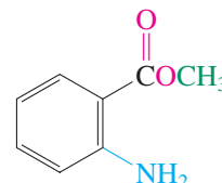
Methyl 2-aminobenzoate (Methyl anthranilate) (A component of grape flavor)
