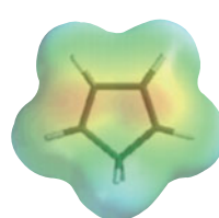
1,3-Cyclopentadiene
