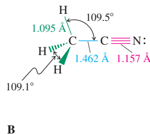
Figure 20-3 (A) Orbital picture of the nitrile group, showing the sp hybridization of both atoms in the \text{C}\equiv\text{N} function. (B) Molecular structure of ethanenitrile (acetonitrile), which is similar to that of the corresponding alkyne. (C) Electrostatic potential map of ethanenitrile, depicting the positively polarized cyano carbon (blue) and the relatively negatively polarized nitrogen (green) with its lone electron pair (red).
