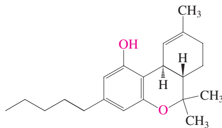
Tetrahydrocannabinol
