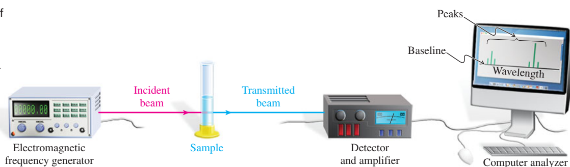
Figure 10-3 General diagram of a spectrometer. Electromagnetic radiation passes through and interacts with a sample by absorption at certain frequencies. The incident beam is altered to a transmitted beam and the changes detected, amplified, and processed by computer to generate a spectrum.
