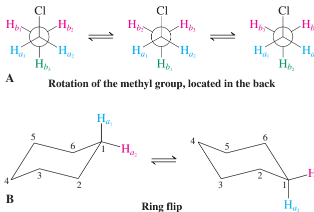
Figure 10-14 (A) Newman projections of chloroethane. In the initial conformation, H_{b1} and H_{b2} are located gauche and H_{b3} anti to the chlorine, and therefore are not in the same environments. However, fast rotation moves each type of H through all positions, thus averaging all the methyl hydrogens on the NMR time scale. (B) In any given conformation of cyclohexane, the axial hydrogens are different from the equatorial ones. However, conformational flip is rapid on the NMR time scale, equilibrating axial and equatorial hydrogens, so only one average signal is observed. Colors are used here to distinguish among environments and thus to indicate distinct chemical shifts.
