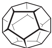
Strain = 61 \text{ kcal mol}^{-1} Dodecahedrane ( \text{C}_{20}\text{H}_{20} )
