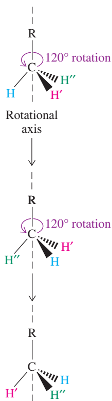
Figure 10-12 Rotation of a methyl group as a test of symmetry.
