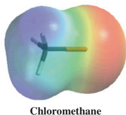
Chloromethane
