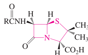
Penicillin
