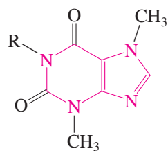
Caffeine (R = CH 3 )
