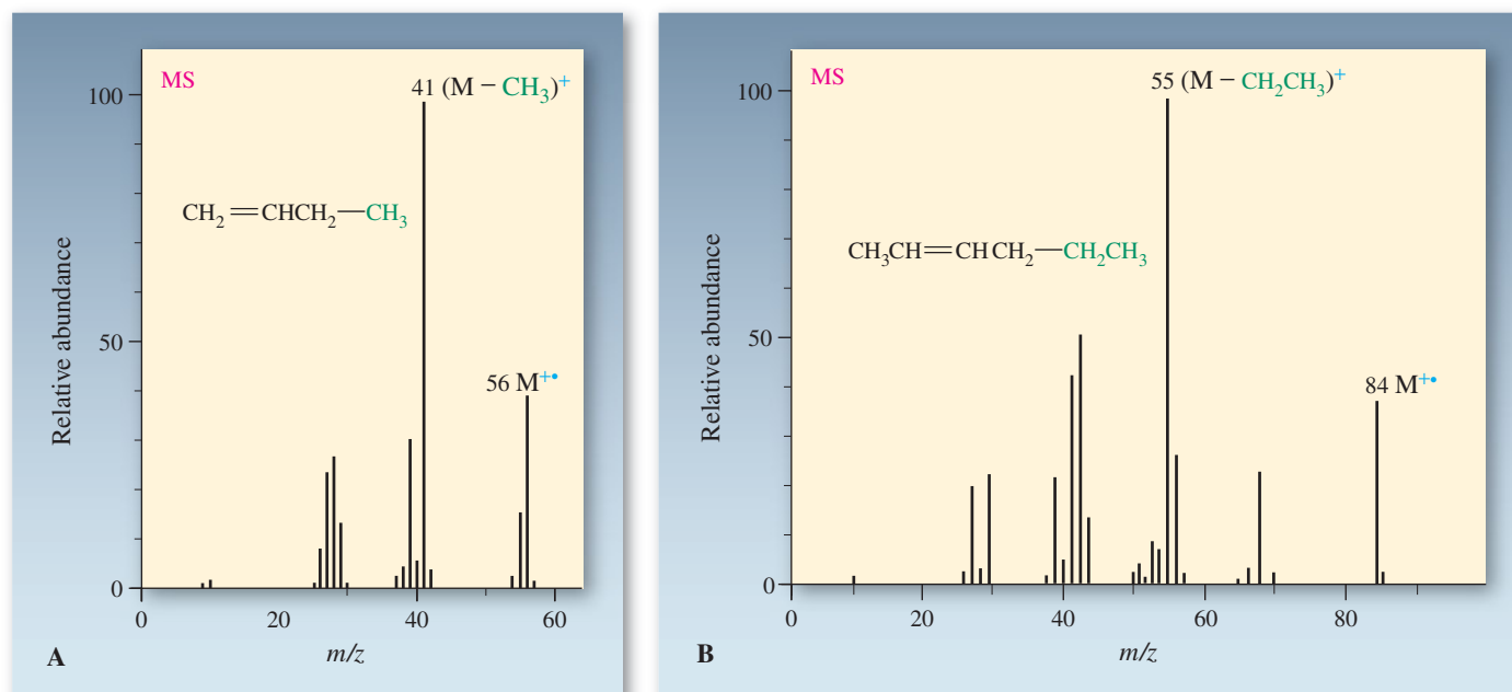
Figure 11-29 Mass spectra of (A) 1-butene, showing a peak at m/z = 41 from cleavage to give the resonance-stabilized 2-propenyl (allyl) cation; (B) 2-hexene, showing similar cleavage between C4 and C5 to give the 2-butenyl cation, with m/z = 55 .
