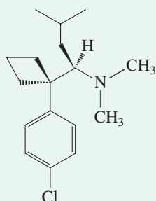
Sibutramine (Meridia)
