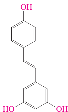
Resveratrol
