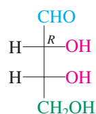
Structure 1 (D-Erythrose)
