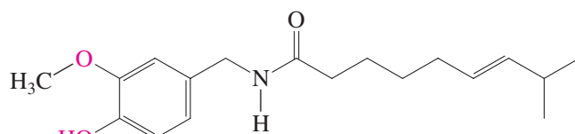
Capsaicin
