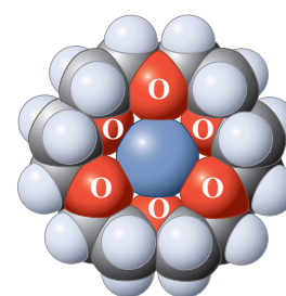
Space-filling model of the cation [\text{K}^+ \text{ 18-crown-6}] .
