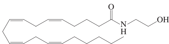
Anandamide
