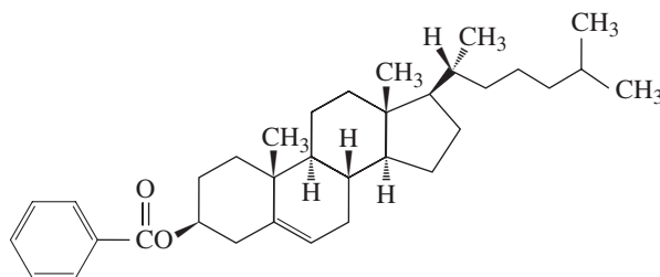
Cholesteryl benzoate
