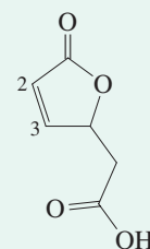
Model compound
