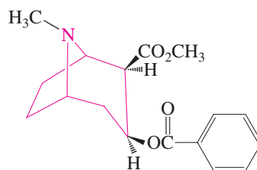
Cocaine
