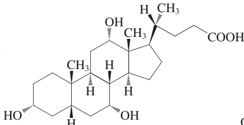
Cholic acid
