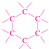
A carbocycle
