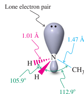
Figure 21-1 Nearly tetrahedral structure of methanamine (methylamine).
