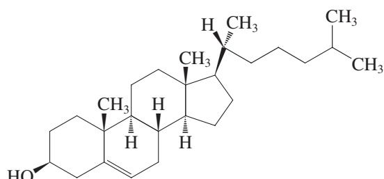
Cholesterol
