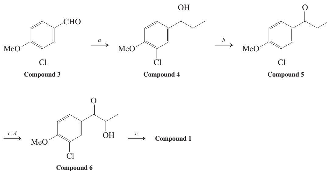
Figure 2 Synthesis of Compound 1; key: (a) standard procedure; (b) PDC, \text{CH}_2\text{Cl}_2 , rt.; (c) \text{TMSCl} , \text{Et}_3\text{N} , rt.; (d) cat. \text{OsO}_4 , NMMO, acetone, 0^\circ\text{C} ; (e) \text{Zn}(\text{BH}_4)_2 , ether, 0^\circ\text{C} .
