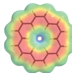
[18]Annulene: aromatic
