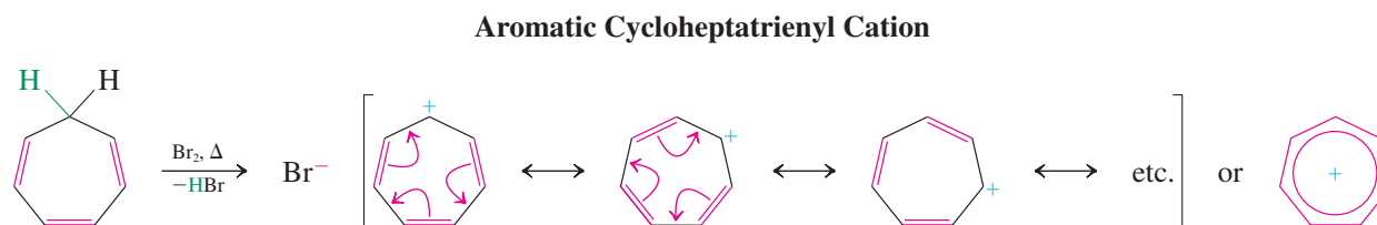
Cycloheptatrienyl cation: aromatic
