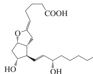
Prostacyclin I_2
