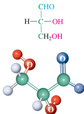
2,3-Dihydroxypropanal (Glyceraldehyde) (An aldotriose )
