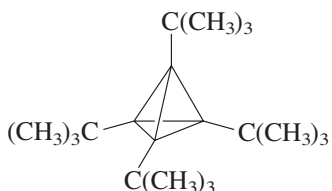
Strain = 129 \text{ kcal mol}^{-1} Tetrakis(1,1-dimethylethyl)- tetrahedrane
