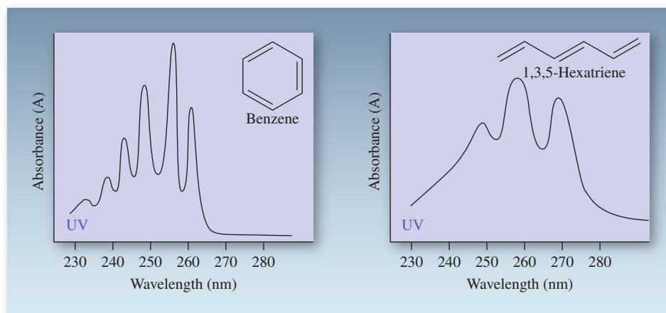
Figure 15-6 The distinctive ultraviolet spectra of benzene: \lambda_{\text{max}}(\epsilon) = 234(30), 238(50), 243(100), 249(190), 255(220), 261(150) \text{ nm} ; and 1,3,5-hexatriene: \lambda_{\text{max}}(\epsilon) = 247(33,900), 258(43,700), 268(36,300) \text{ nm} . The extinction coefficients \epsilon of the absorptions of 1,3,5-hexatriene are very much larger than those of benzene; therefore the spectrum at the right was taken at lower concentration.
