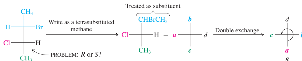
Figure 5-8 Assigning the absolute configuration at C3 in 2-bromo-3-chlorobutane. We consider the group containing the stereocenter C2 merely as one of the four substituents. Priorities (also noted in color) are assigned in the usual way ( \text{Cl} > \text{CHBrCH}_3 > \text{CH}_3 > \text{H} ), giving rise to the representation shown in the center. Two exchanges place the substituent of lowest priority (hydrogen) at the top of the Fischer projection to facilitate assignment.
