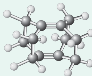
Molecular model of D
