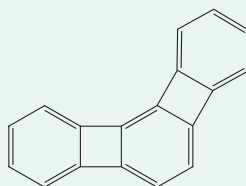
B Angular [3]phenylene
