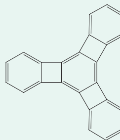
C C_3 -symmetric [4]phenylene
