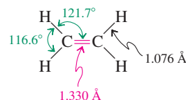
Figure 11-1 Molecular structure of ethene.
