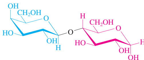
Crystalline \alpha -lactose, a \beta -D-galactopyranosyl- \alpha -D-glucopyranose
