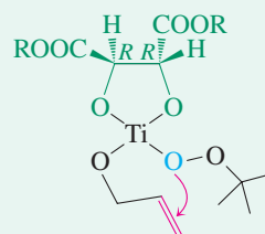
Transition State for R,R -Tartrate
