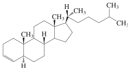
3-Cholestene
