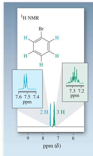
Figure 15-10 A part of the 300-MHz 1 H NMR spectrum of bromobenzene, a non-first-order spectrum.
