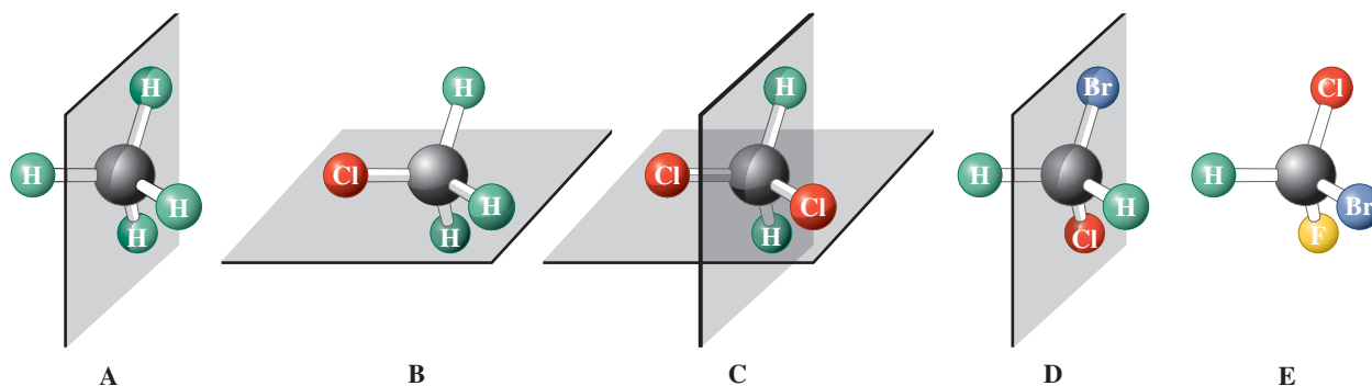
Figure 5-4 Examples of planes of symmetry: (A) methane has six planes of symmetry (incorporating the six edges of the tetrahedral frame), only one of which is shown; (B) chloromethane has three such planes, only one of which is shown; (C) dichloromethane has only two; (D) bromochloromethane only one; and (E) bromochlorofluoromethane has none. Chiral molecules cannot have a plane of symmetry.
