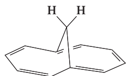
1,6-Methano[10]annulene
