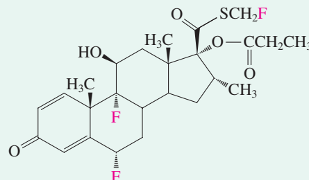
Fluticasone propionate
