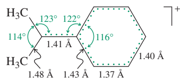
Figure 22-2 Structure of the 2-phenyl-2-propyl cation.
