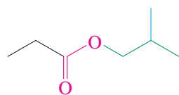
2-Methylpropyl propanoate (Isobutyl propionate) (A component of rum flavor)
