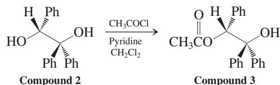
Figure 1 Synthesis of Compound 3 (Ph = phenyl, \text{C}_6\text{H}_5 ).
