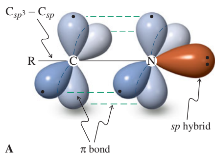
Figure 20-3 (A) Orbital picture of the nitrile group, showing the sp hybridization of both atoms in the \text{C}\equiv\text{N} function. (B) Molecular structure of ethanenitrile (acetonitrile), which is similar to that of the corresponding alkyne. (C) Electrostatic potential map of ethanenitrile, depicting the positively polarized cyano carbon (blue) and the relatively negatively polarized nitrogen (green) with its lone electron pair (red).
