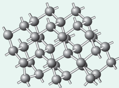
Diamond
