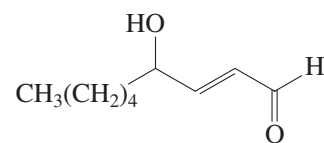
trans -4-Hydroxy-2-nonenal
