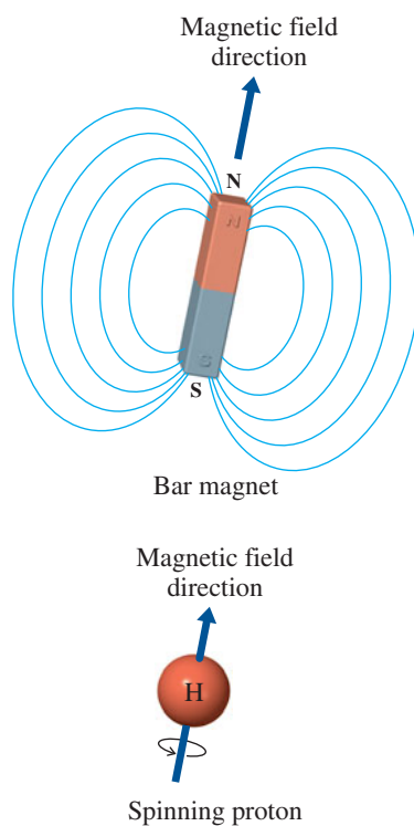
The Spinning Proton Creates a Magnetic Field
