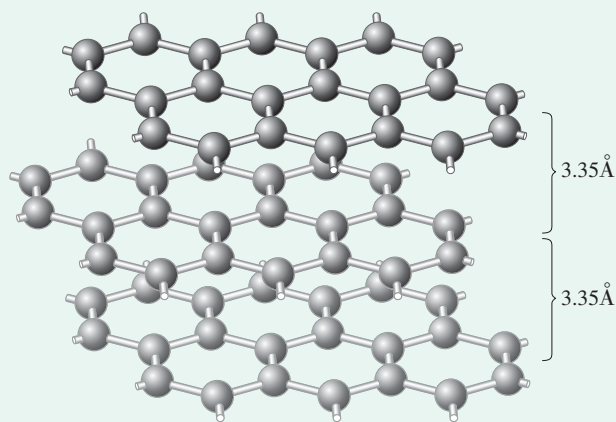
Graphite
