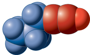
Propylacetylene
