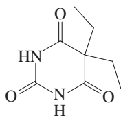
Veronal
