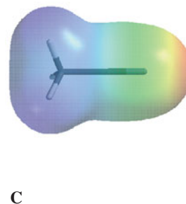
Figure 20-3 (A) Orbital picture of the nitrile group, showing the sp hybridization of both atoms in the \text{C}\equiv\text{N} function. (B) Molecular structure of ethanenitrile (acetonitrile), which is similar to that of the corresponding alkyne. (C) Electrostatic potential map of ethanenitrile, depicting the positively polarized cyano carbon (blue) and the relatively negatively polarized nitrogen (green) with its lone electron pair (red).
