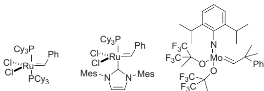
Grubbs' catalysts
